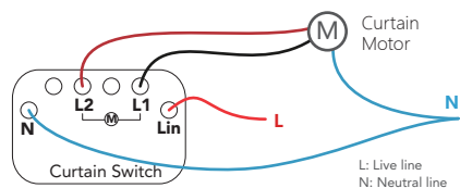
Diagram 1: For 1 Gang curtain switches
